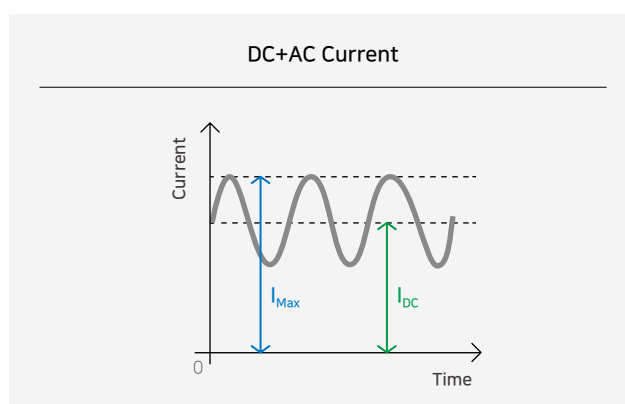
[Types of current applied to the inductor]
