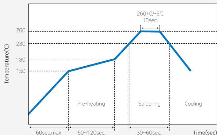
[Reflow Soldering Conditions]
