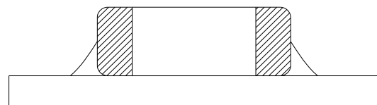
Not enough solder Weak holding force may cause bad connections or detaching of the power inductor
