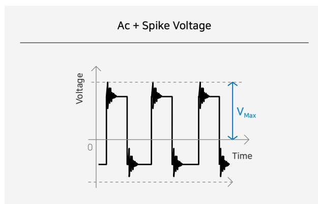
[Types of voltage applied to the inductor]
