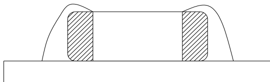
Too Much Solder large stress may cause damages
