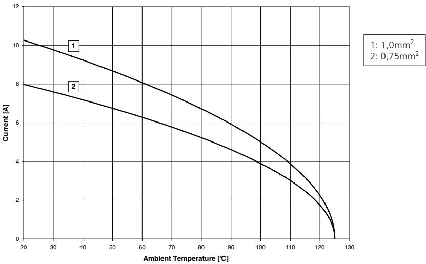
Derating Curve
