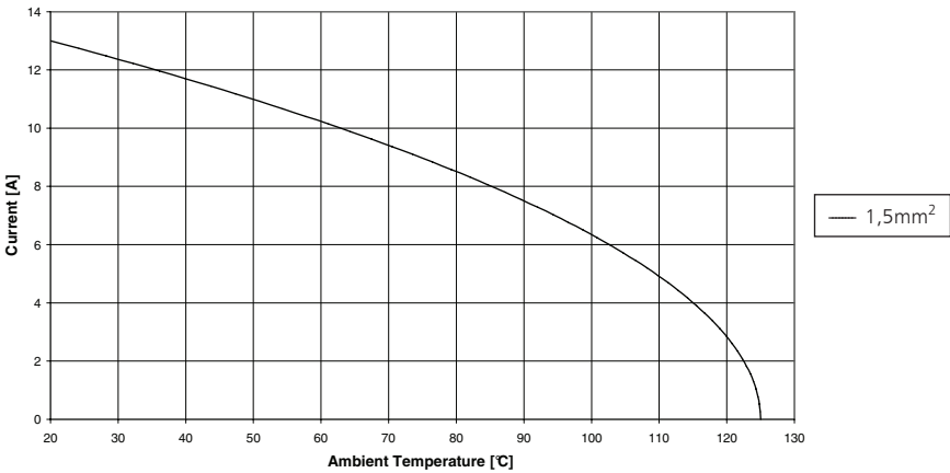
Derating Curve
