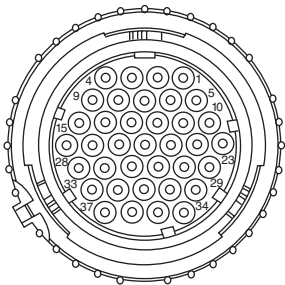
Coding 37-way layout View on Mating Face
