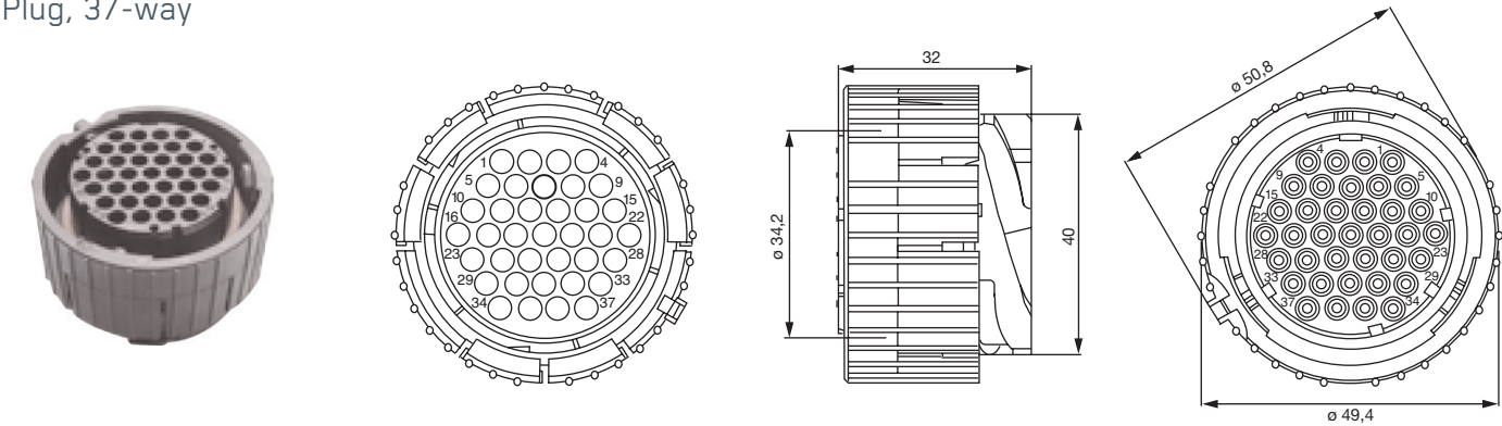
Plug, 37-way
