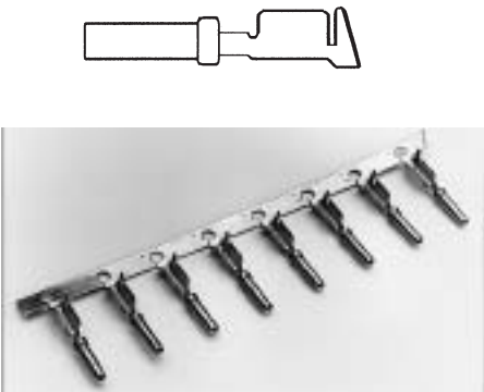
Hooded Socket
