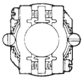
Cable connecting plug MS 3101E and F/CA 3101E Dimensions/sizes
