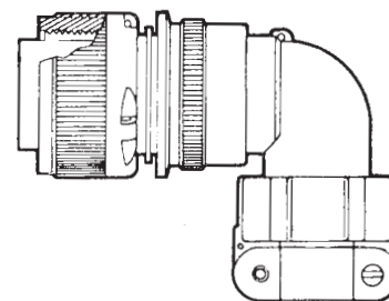
90° Angle plug MS 3108E and R/CA 3108E/F/R 1)
