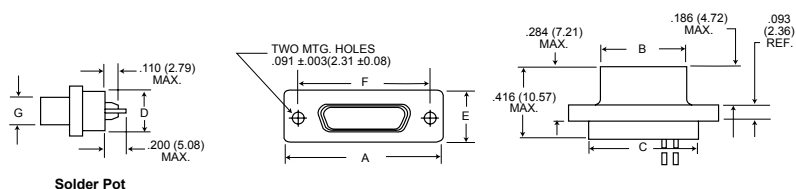
Solder Pot
