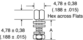
Front Panel Mount
