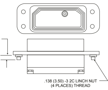
Mounting Style F Clinch Nut Mounting
