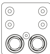
7W2 1 #16 4 #12 2 #5 Coax
