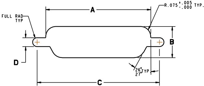
Rear Mounting
