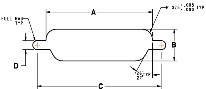
Rear Mounting
