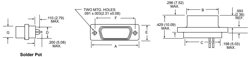
Solder Pot
