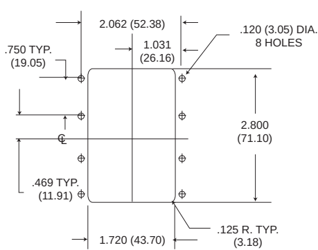
- 33 FRONT MOUNT
