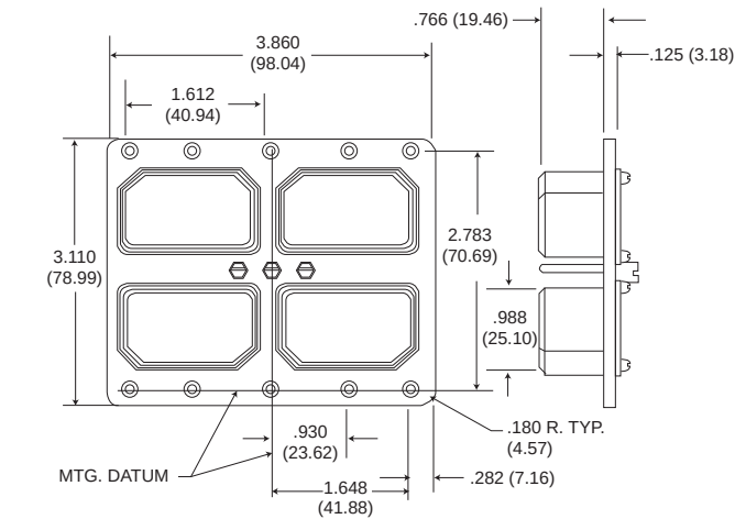
DPX4-33
