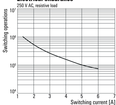
Electrical endurance
