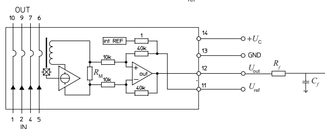
Figure 17: filtered U_{\text{out}} connection
