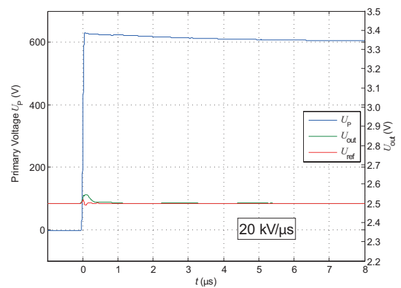
Figure 10: du/dt
