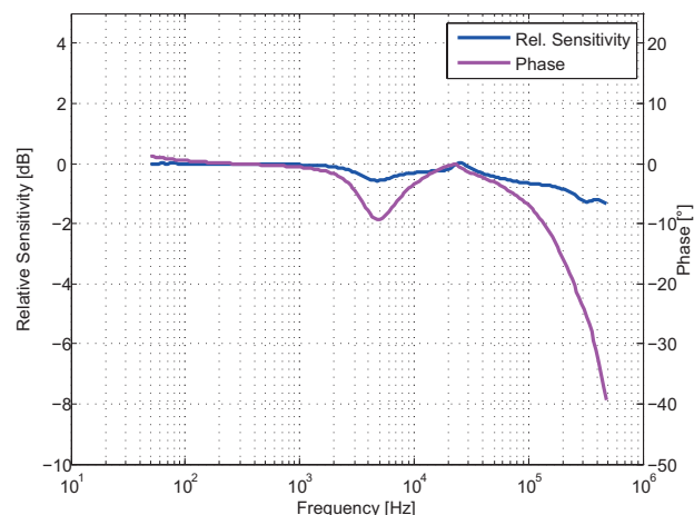
Figure 2: Frequency response
