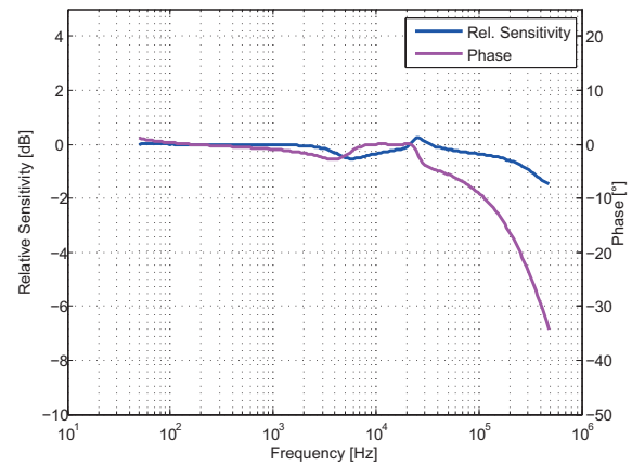
Figure 7: Frequency response
