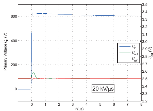
Figure 5: du/dt
