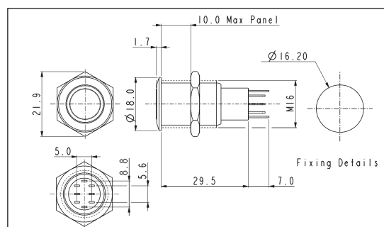
Contact Layout
