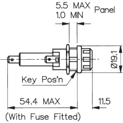
Fixing Detail
