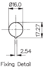
Fixing Detail
