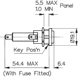
Fixing Detail
