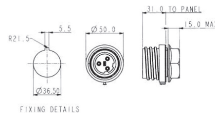
FIXING DETAILS
