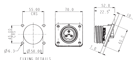
FIXING DETAILS
