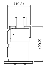
Inner-housing lock
