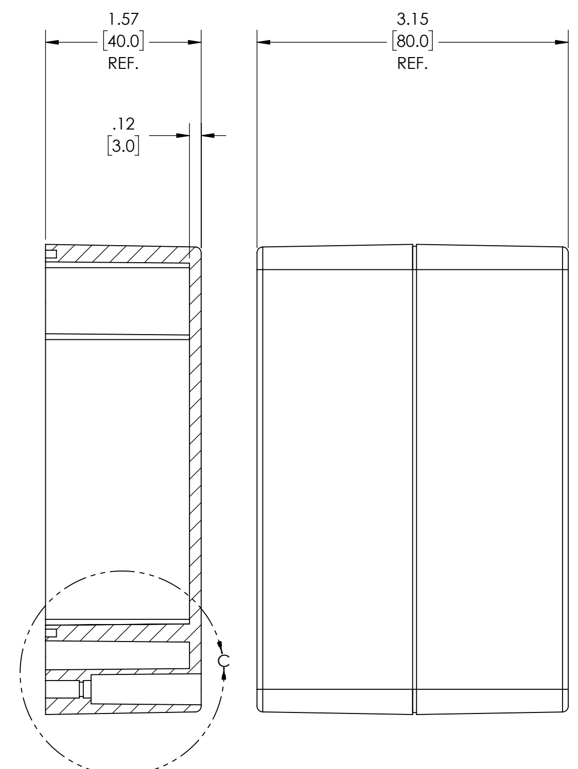
SECTION B-B
