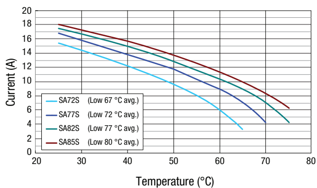
Current vs. Temperature Curves S-Type
