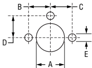
Suggested Panel Layout
