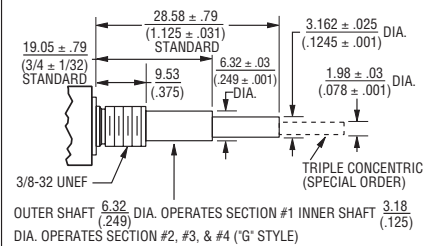
"C" Bushing 1/4" (6.35 mm) Dia. Plain - Concentric Shaft
