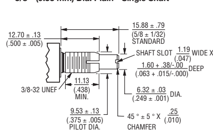
"B" Bushing 3/8" (9.53 mm) Dia. Plain - Single Shaft
