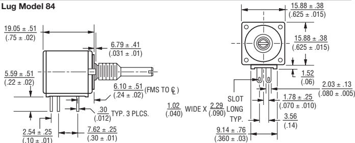
"A" Bushing 3/8" (9.53 mm) Dia. Plain - Single Shaft
