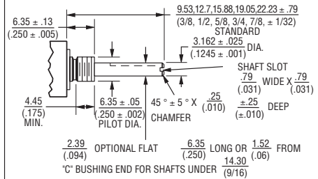
"E" Bushing 1/4" (6.35 mm) Dia. Locking - Single Shaft
