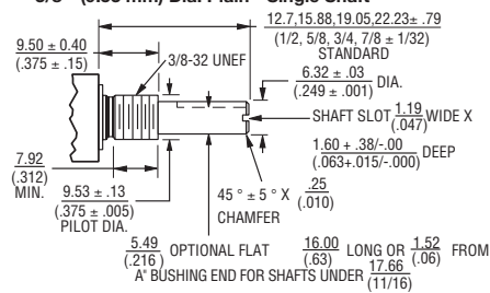
"B" Bushing 3/8" (9.53 mm) Dia. Plain - Single Shaft
