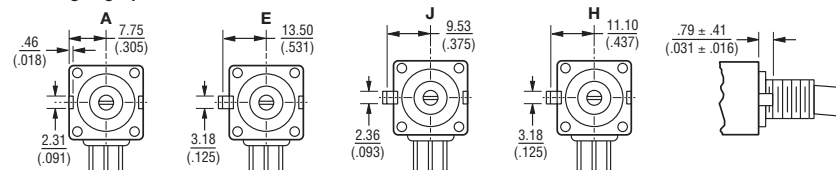
Locating Lug Options - All Model 80 Series
