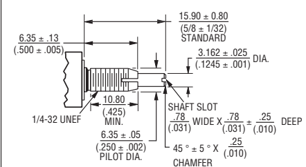
"A" Bushing 3/8" (9.53 mm) Dia. Plain - Concentric Shaft
