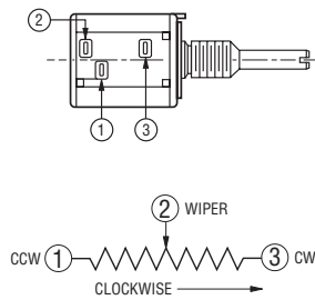
Shaft Flat Orientation
