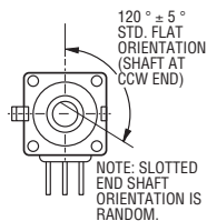
Shaft Flat Orientation
