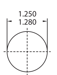
MOUNTING HOLE AG
