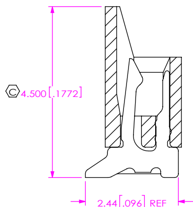
-03 LEAD STYLE IN PROCESS 1A FILL C-297-04-T (SAME AS IN PROCESS 1 FOR -01 LEAD STYLE EXCEPT AS SHOWN) (ODD POSITIONS FILLED ONLY)
