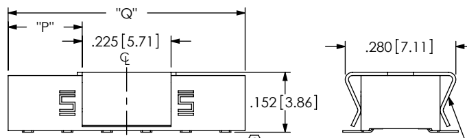
FIGURE 5 (-P: PICK & PLACE PAD)
