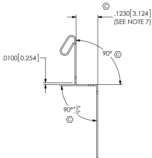
IN-PROCESS 2 (FORM BOTTOM ROW) (C-150-05-X-P SHOWN) (-RA2 ONLY)
