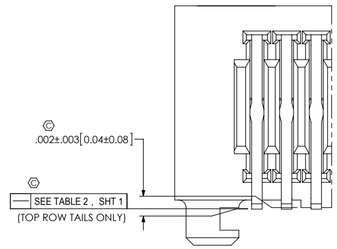
DETAIL 'H' SCALE 8:1
