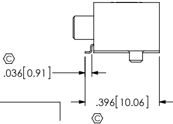
IN-PROCESS 4 (SHEAR BOTTOM ROW)
