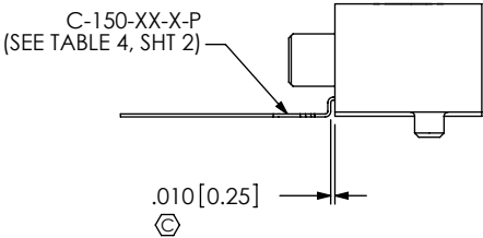
IN-PROCESS 3 (FILL BOTTOM ROW)
