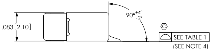
FIG 1 ZF5-20-01-X-WT SHOWN (WITH CAM CLOSED)
