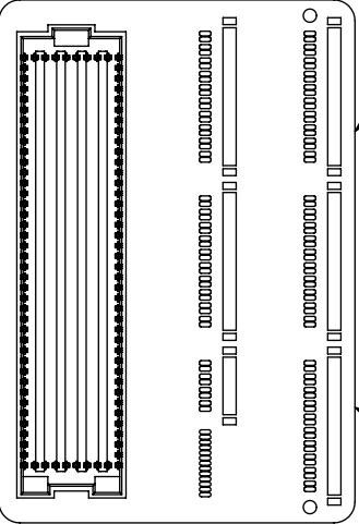
J1 SUB-HDR-153208-01
