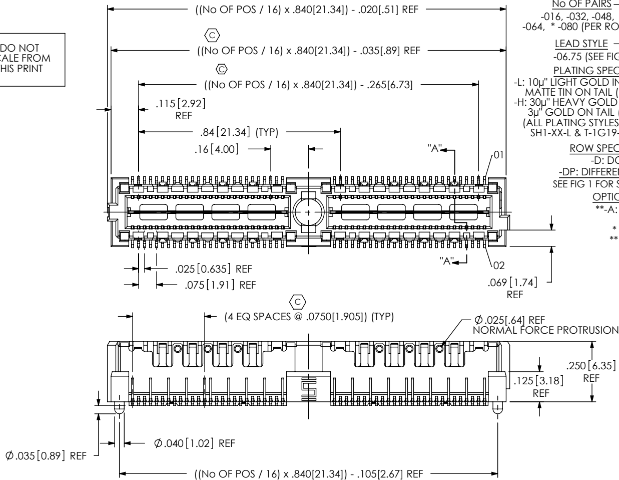
FIG 1 -06.75 LEAD STYLE (QMSS-032-06.75-X-D-DP-A SHOWN) (MATED HEIGHT WITH QFSS-04.25: .433 [11.00] REF)
