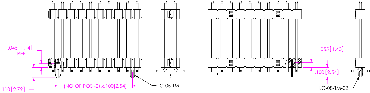
FIG 2 -LC: LOCKING CLIP (SAME AS FIG 1, DIFFERENT AS SHOWN)
