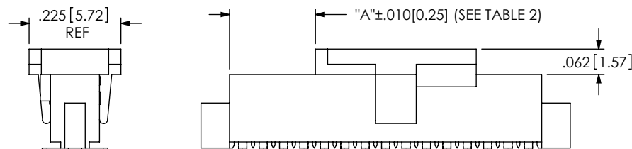
FIG 5 -P: PICK AND PLACE PAD (PAD TO BE ORIENTED A SHOWN FOR 5-12 POSITION PARTS) (FOR 13-50 POSITION PARTS, PAD MAY BE ORIENTED IN EITHER DIRECTION) (SAME AS FIG 1, DIFFERENT AS SHOWN)
