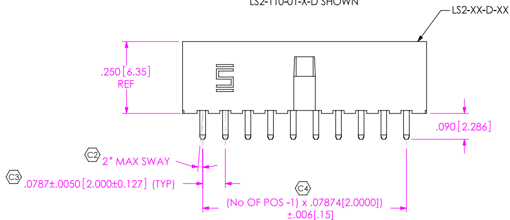
FIG. 1 LS2-110-01-X-D SHOWN
