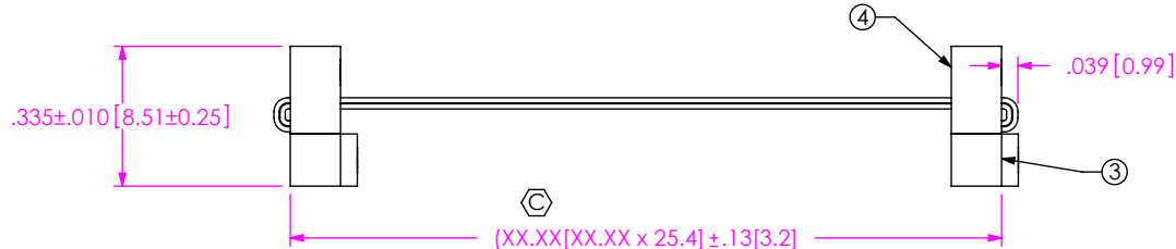
FIG 9 STRAIN RELIEF OPTION (POS 2-15 ONLY) (FFSD-10-D-XX.XX-01-X-N-SR SHOWN) (SAME AS FIG 1, DIFFERENT AS SHOWN)
