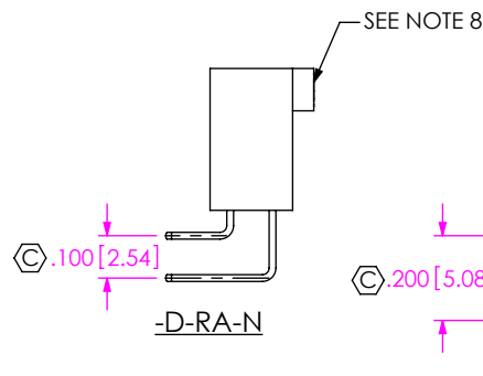
FIG 2 RIGHT ANGLE OPTION ALL OPTIONS DIFFERENT AS SHOWN, OTHERWISE SAME AS -S-RA
