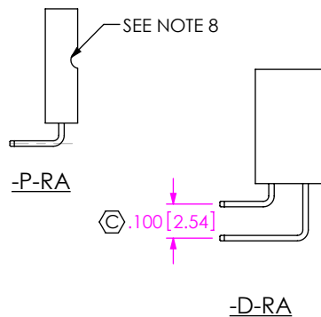
FIG 2 RIGHT ANGLE OPTION ALL OPTIONS DIFFERENT AS SHOWN, OTHERWISE SAME AS -S-RA
