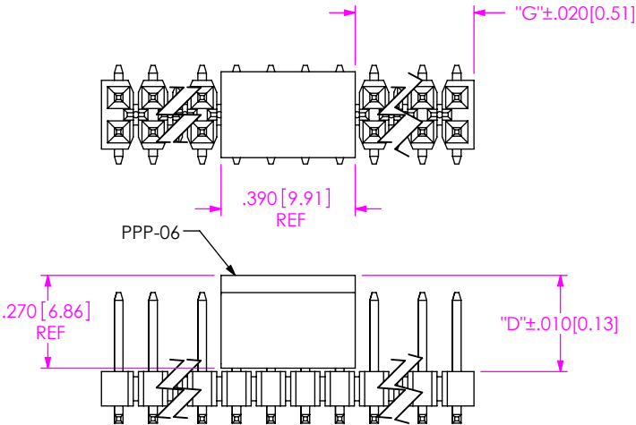
FIG 4 -P: PICK AND PLACE PAD (DIFFERENT AS SHOWN, OTHERWISE SAME AS FIG 1) "G" = ((\text{NO OF POS} \times .100 [2.54]) - .390 [9.91]) / 2
