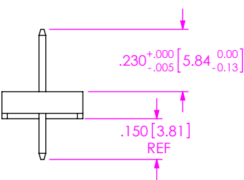
IN-PROCESS 1 -TV MOUNT STYLE
