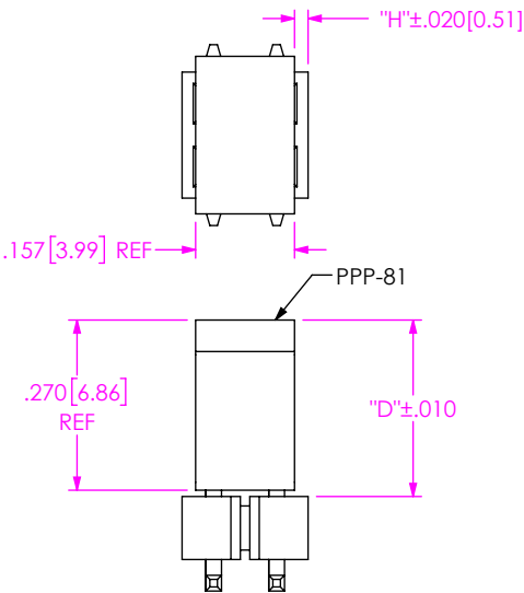
FIG 9 -P: PICK AND PLACE PAD (-02 & -03 POS ONLY) (DIFFERENT AS SHOWN, OTHERWISE SAME AS FIG 1) "H" = ((\text{NO OF POS} \times .100 [2.54]) - .157 [3.99]) / 2
