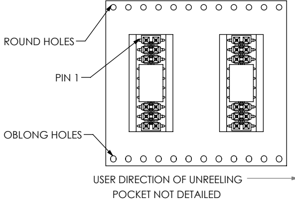
FIG 8 PACKAGING VIEWS
