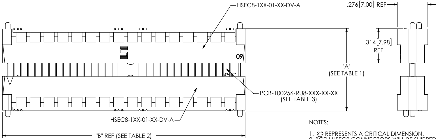
FIG 1 RU8-160-19-SE-XX-DV SHOWN
