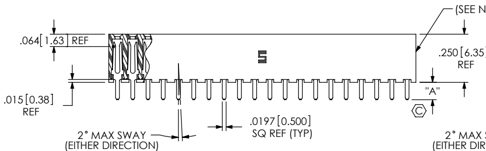
FIG 1 SQT-120-01-XX-6 SHOWN
