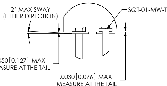
DETAIL 'B' SCALE 6:1
