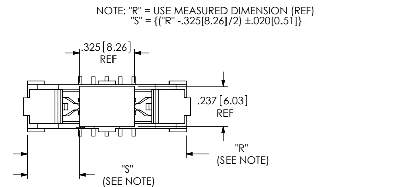
FIG 3 (EHT-105-01-XX-D-SM-K SHOWN) -K OPTION (POLYIMIDE FILM PAD) (DIFFERENT AS SHOWN, OTHERWISE SAME AS FIG 1)
