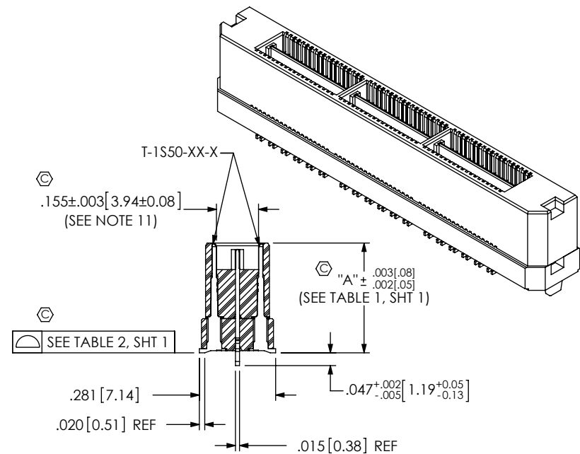
SECTION "B"-"B"
