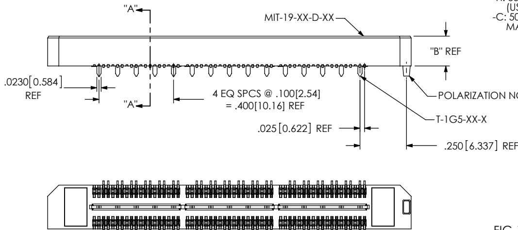
FIG 1 -01 LEAD STYLE (MIT-036-01-X-D-DP SHOWN) (STYLE -01 & -02 ONLY)
