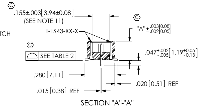
FIG 1 -01 LEAD STYLE (MIT-036-01-X-D-DP SHOWN) (STYLE -01 & -02 ONLY)
