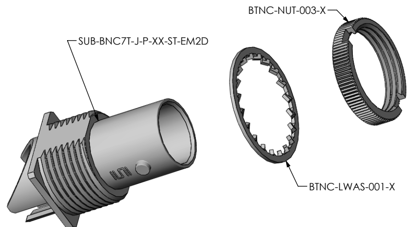
FIG 1 BNC7T-J-P-XX-ST-EM2D SHOWN
