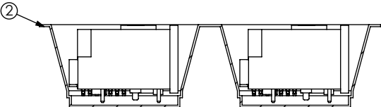
PACKAGING VIEW
