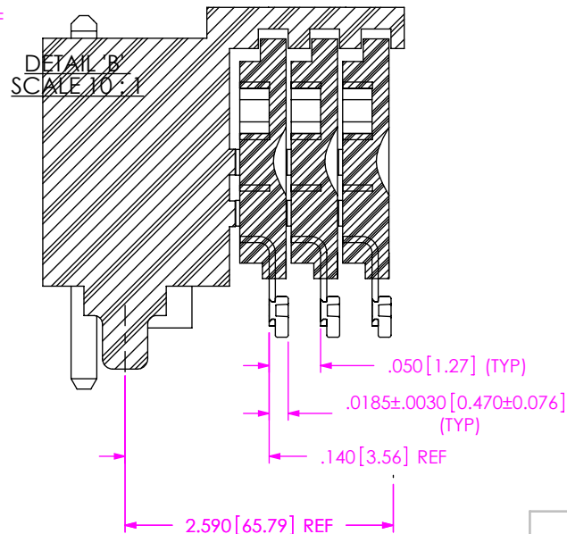
SECTION "F"-"F" SCALE 6:1
