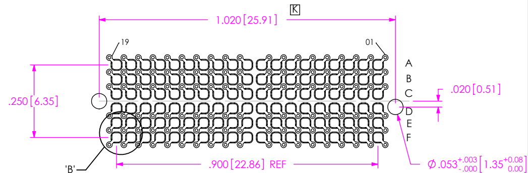
RECOMENDED BOARD LAYOUT
