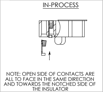
PACKAGING VIEW
