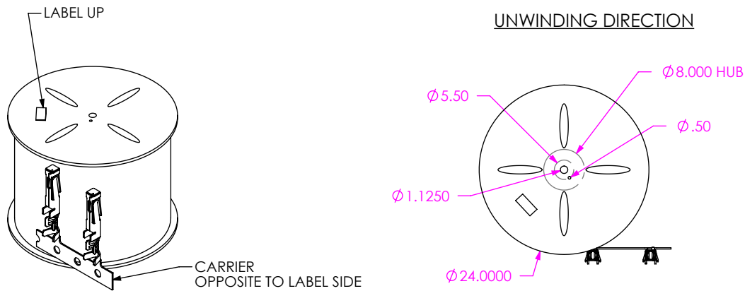
FIG 3 REEL SPECIFICATIONS USE REEL R-24-08.00-1.00-P (SEE NOTE 4)
