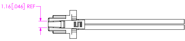
FIG 4 S1SS-02-XXX-XX-XX.XX-L SHOWN (DIFFERENT AS SHOWN, OTHERWISE SAME AS FIG 1) (FOR POSITIONS -02 THRU -04)
