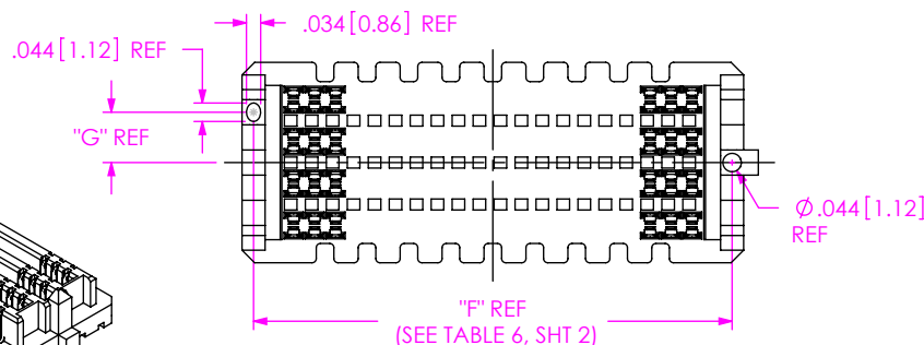
FIG 1 -08: 8 ROW (SEAM-30-02.0-XXX-08-1-A-XX-K-TR SHOWN) (SOME CENTER FEATURES REMOVED FOR CLARITY)
