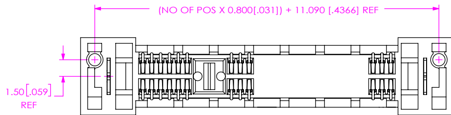
FIG 2 **-L2: ECDP LATCHING OPTION HSEC8-125-01-XX-DV-A-L2 SHOWN (AVAILABLE IN 9, 13, 25, & 49 POS ONLY) (NOT AVAILABLE FOR -GR TYPE USE) (DIFFERENT AS SHOWN, OTHERWISE SAME AS FIG 2) (SOME FEATURES NOT SHOWN FOR CLARITY) (** = AVAILABLE ONLY WITH -01 CARD THICKNESS)
