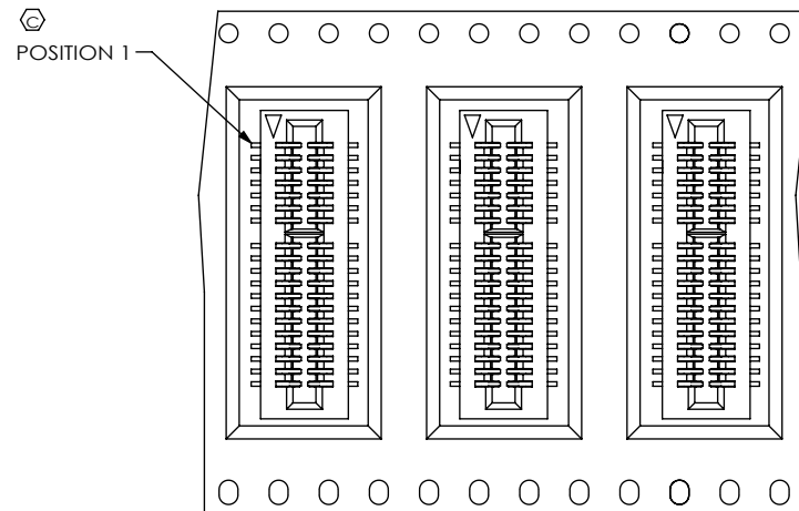
FIG 5 -TR: TAPE & REEL PACKAGING (NOT DRAWN TO SCALE)
