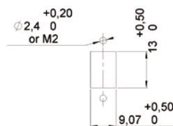
Panel Piercing
