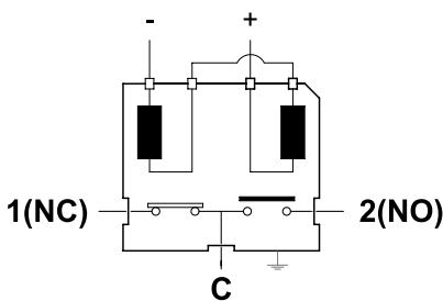
Failsafe model (Type 1)
