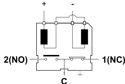
Inverted failsafe model for Bypass application (Type 9)
