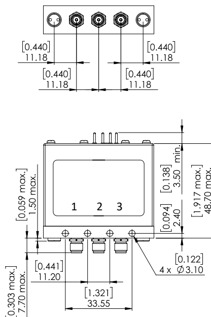
Model SMA2.9 with solder pins
