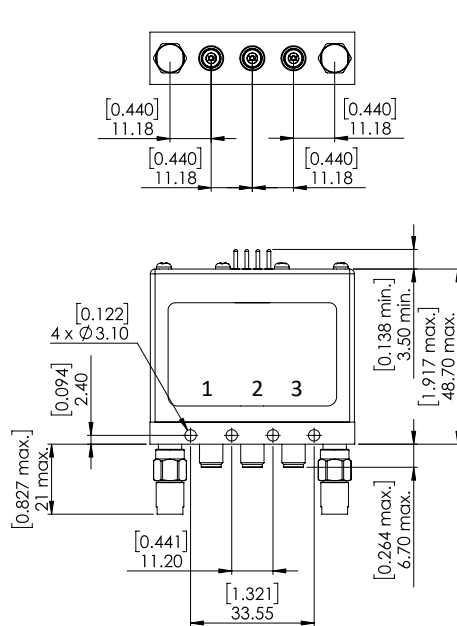
Model SMA2.9 with solder pins
