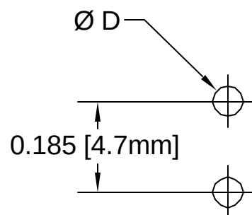
Recommended Mounting Holes
