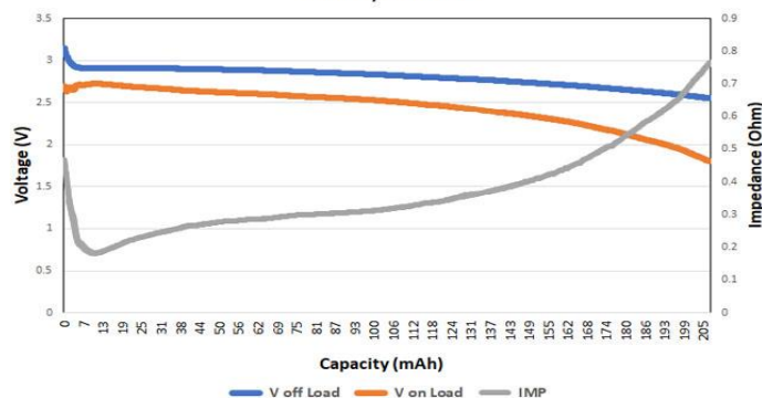
Pulse Discharge Impedance 20mA 1s/14s to 1.8V
