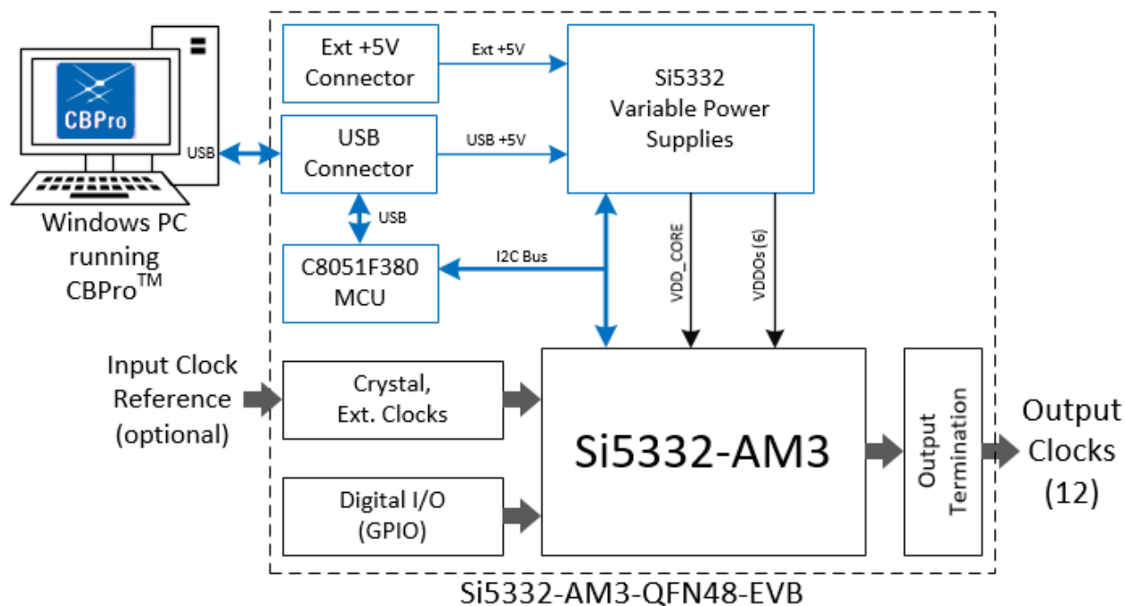
Figure 1.1. Si5332-AM3-QFN48-EVB Functional Block Diagram
