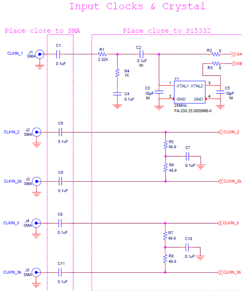
Figure 3.3. Si5332-AM3-QFN48-EVB Input Clock Circuit
